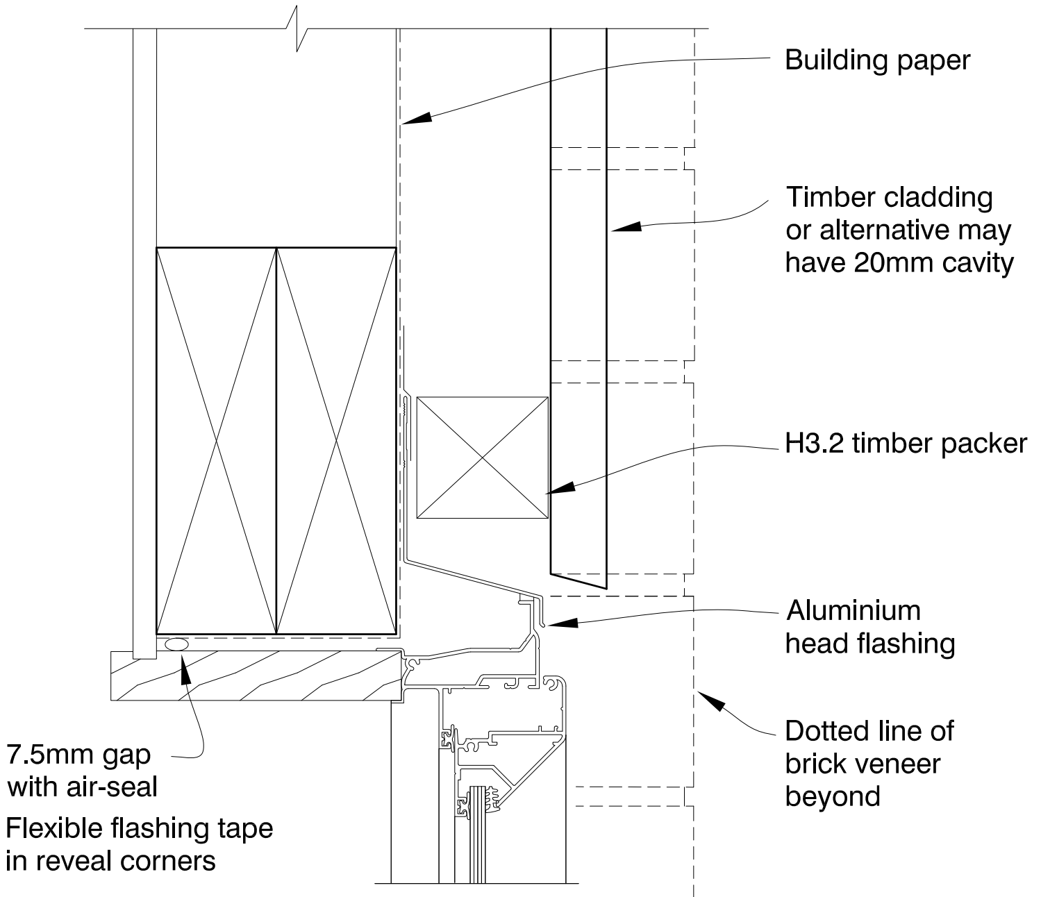
FIG. 28 WINDOW HEAD - ALUMINIUM Alternative cladding above
