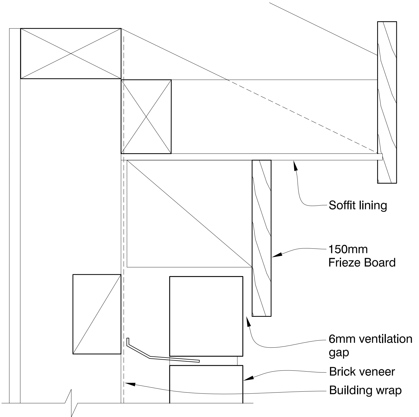
FIG. 82 FLAT SOFFIT & 150mm FRIEZE BOARD
