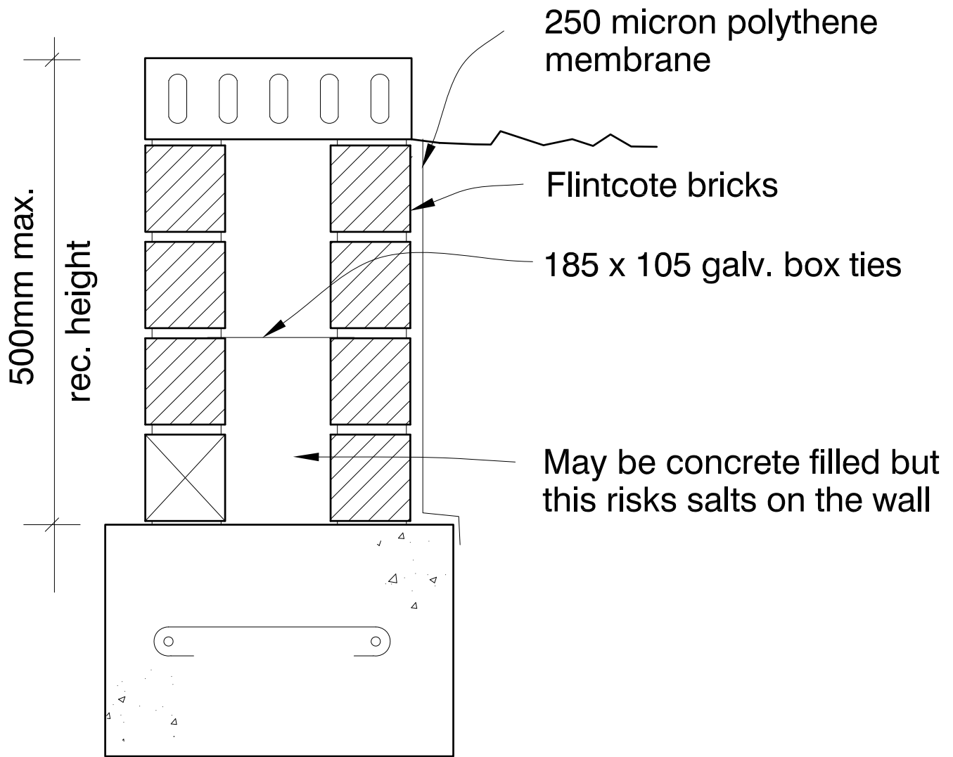
FIG. 116 BRICK EDGING
