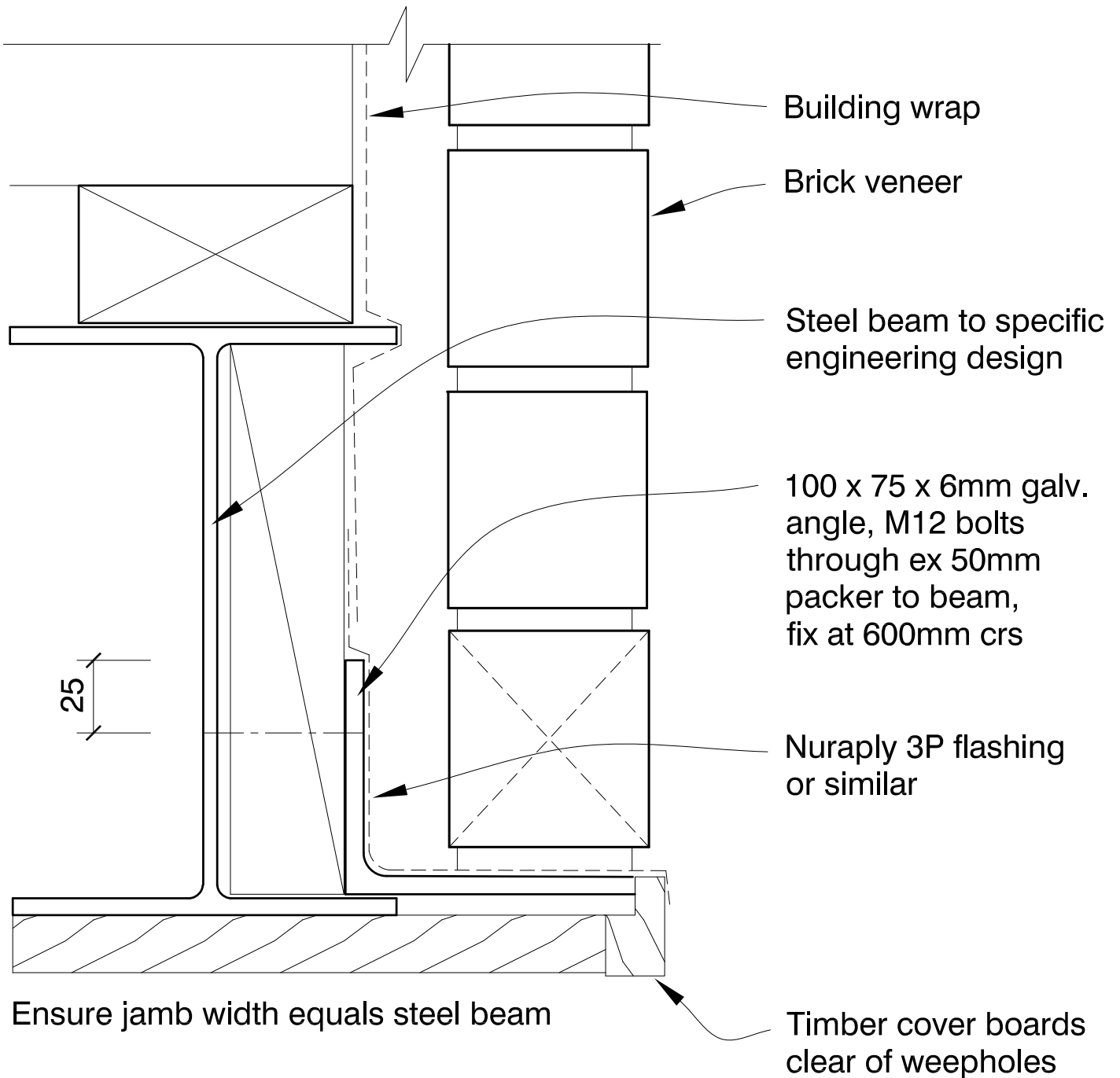
FIG. 49 LARGE WIDTH LINTEL - UB
