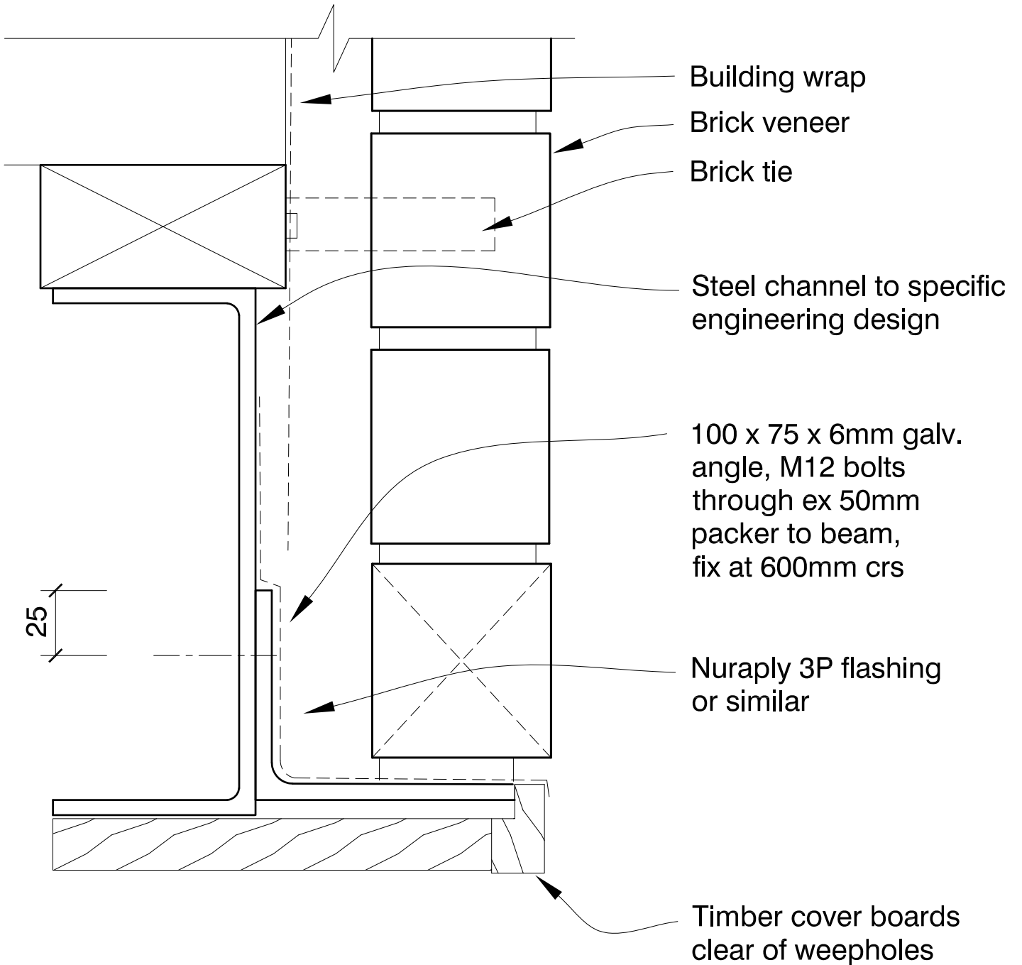
FIG. 50 LARGE WIDTH LINTEL - CHANNEL
