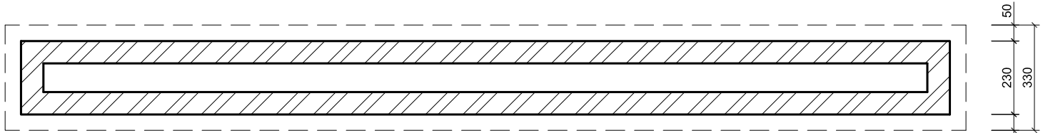
Double Skinned Walls
