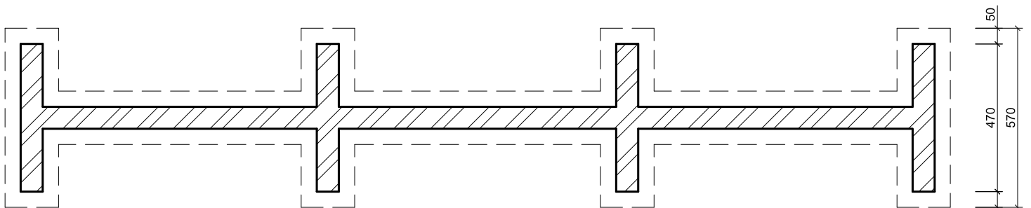
Single Skinned wall with buttresses
