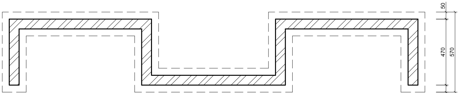
Single Skinned Walls
